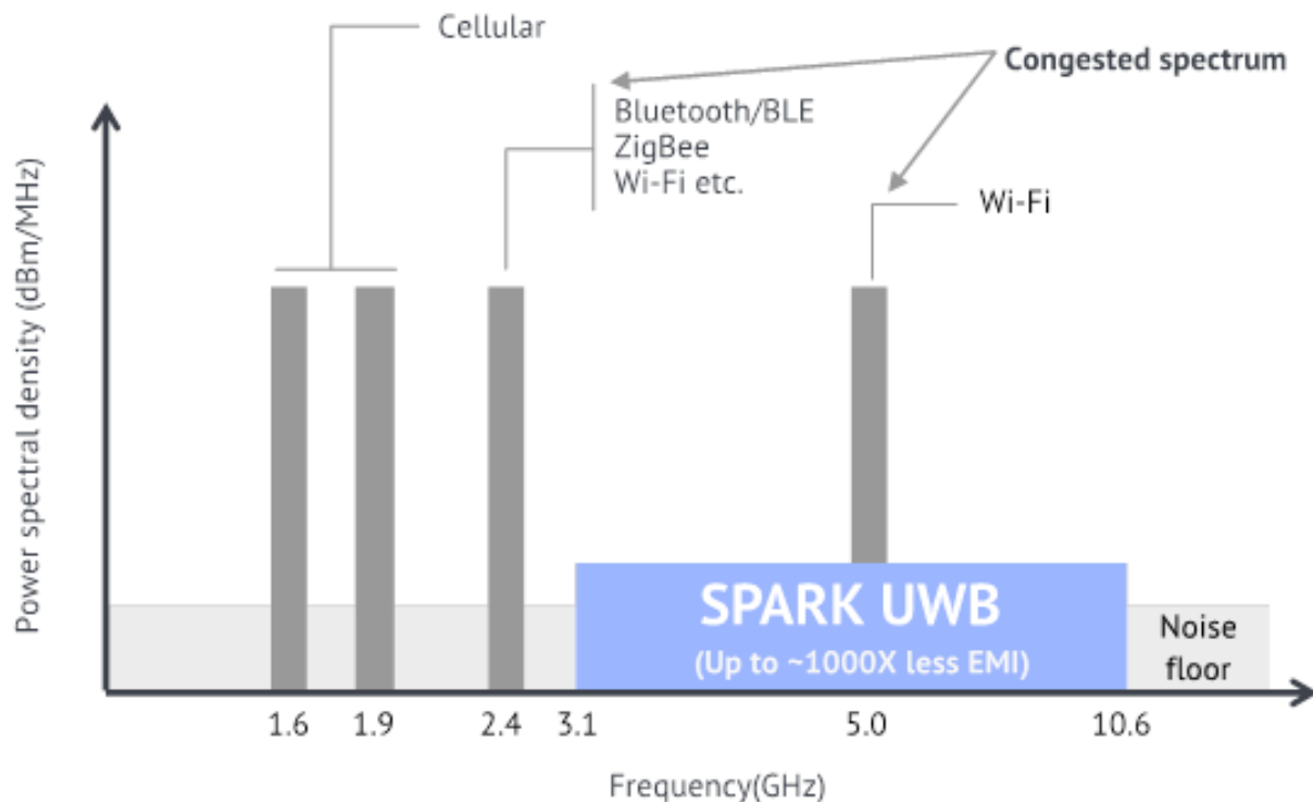
Figure 3: The Frequency Advantage of UWB (source SPARK Microsystems).
