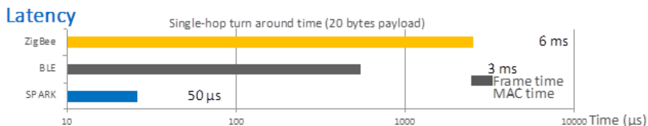
Figure 8: The latency performance provided by the SPARK Microsystems UWB transceiver architecture. (source SPARK Microsystems).
