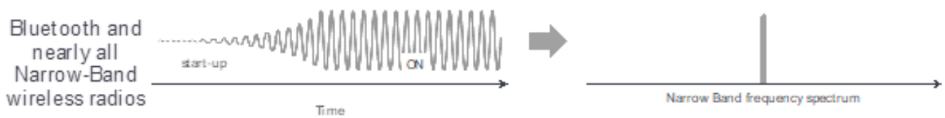
Figure 1: Bluetooth and Narrow-Band radio architecture time and frequency representations.
