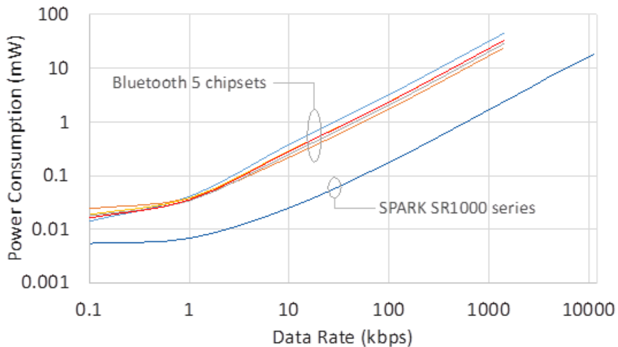
Figure 7: Transmit + receive power consumption profiles of different Bluetooth 5 chipsets and SPARK UWB against data rate. (source SPARK Microsystems).
