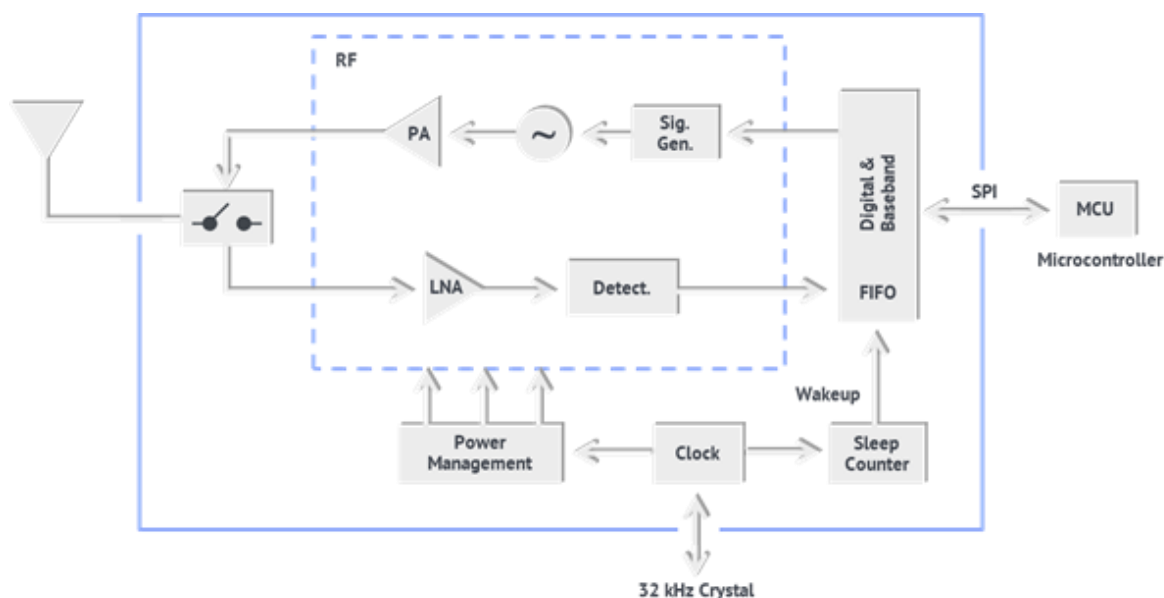
Figure 9: The SPARK Microsystems SR1000 series UWB transceiver functional block diagram. (source SPARK Microsystems).
