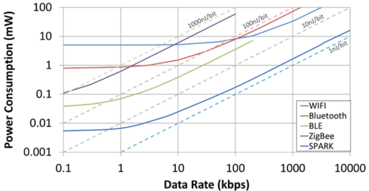
Figure 6: Transmit + receive power consumption profiles of WiFi, Bluetooth, BLE 4.2, ZigBee, and SPARK UWB against data rate. Logarithmic scale. (source SPARK Microsystems).
