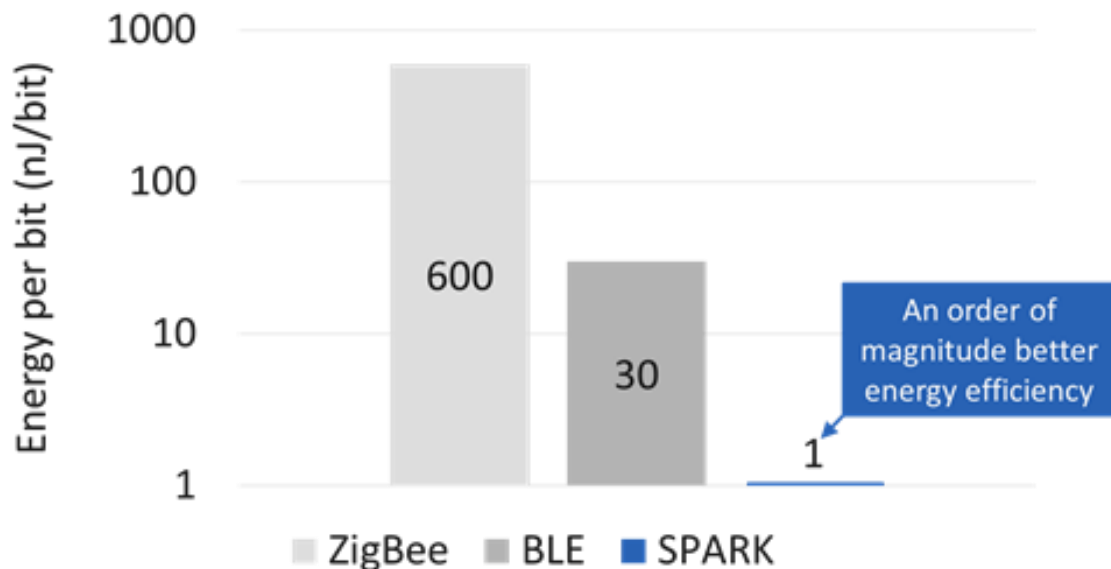
Figure 5: Energy efficiency comparison of energy used to transfer one bit for ZigBee, BLE, and SPARK UWB. Logarithmic scale. (source SPARK Microsystems).
