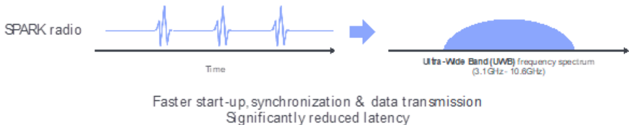
Figure 2: SPARK Microsystems radio architecture time and frequency representations.
