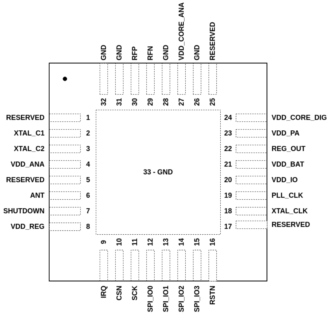
Figure 2.1: QFN32 Package
