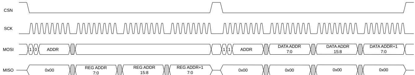
Figure 1.8: SPI burst read and write transaction.
